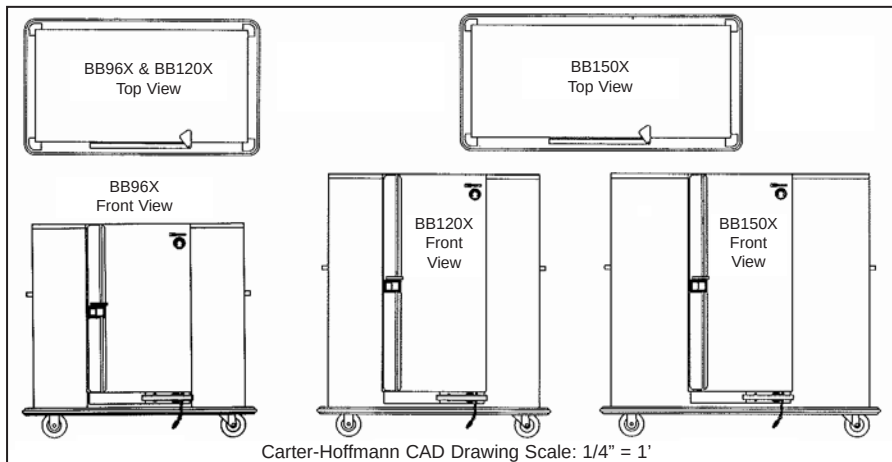
Carter-Hoffmann CAD Drawing Scale: 1/4" = 1'
